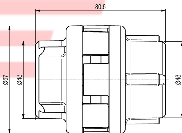
New Flexible Couplings NHD Series
