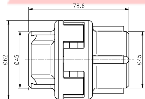
Current Flexible Couplings NHD Series
