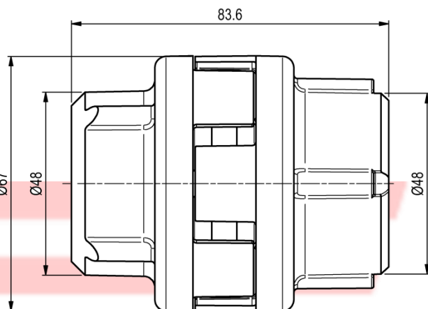
New Flexible Couplings NMT Series
